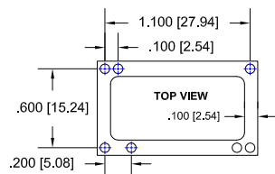
FIG.28 Thru-Hole: C10-624-07-02-01S-R27-L14 Surface Mount: C10-624-07-02-93S-R27-L14
