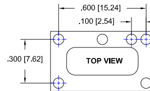
FIG.25 Thru-Hole: C10-314-06-01-01S-R27-L14 Surface Mount: C10-314-06-01-93S-R27-L14
